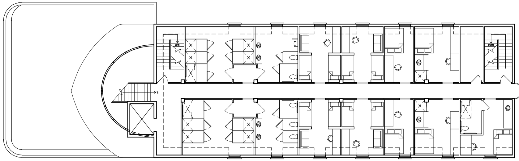
Penthouse/Fourth Floor Plan
